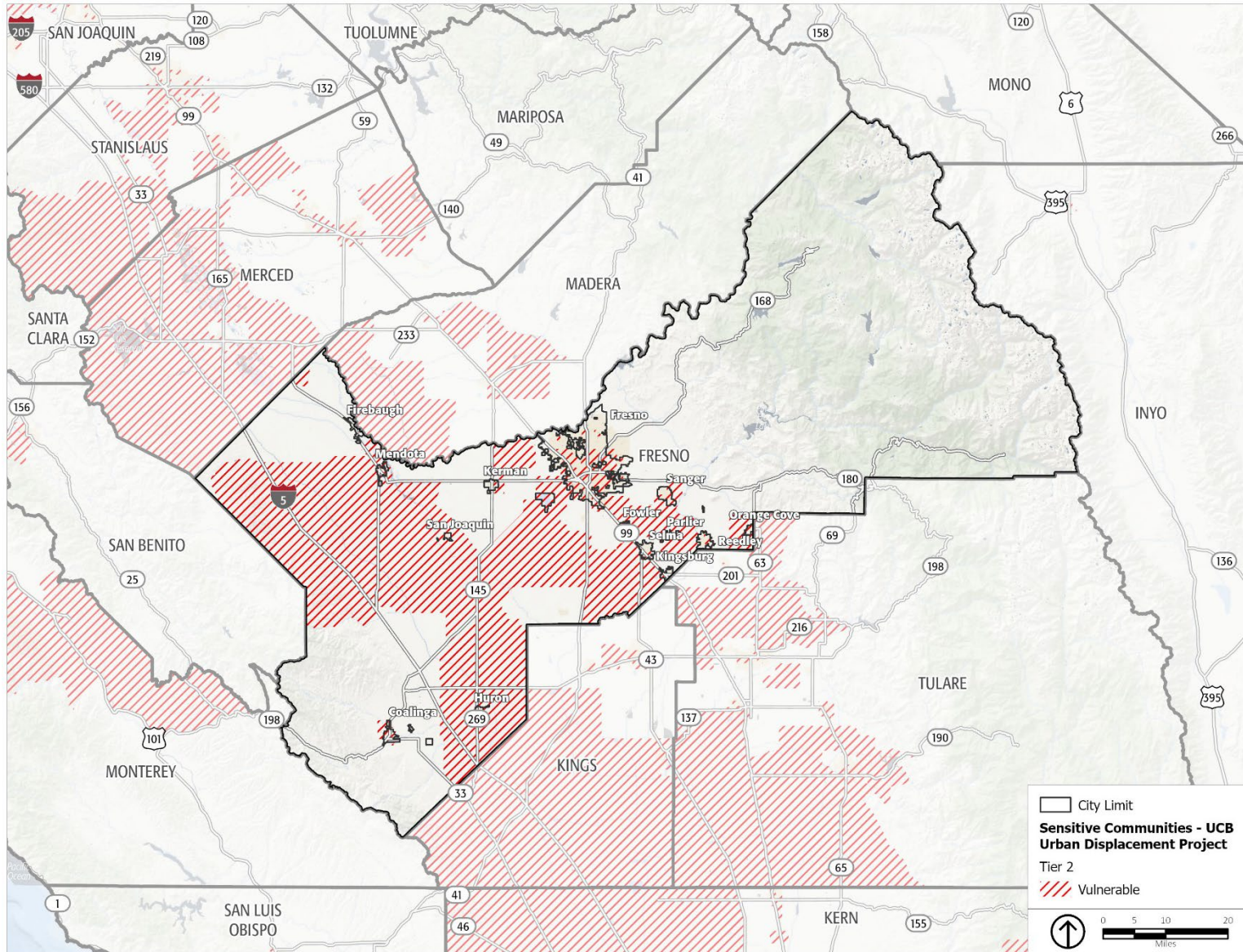
FIGURE 3-38 SENSITIVE COMMUNITIES, 2020
