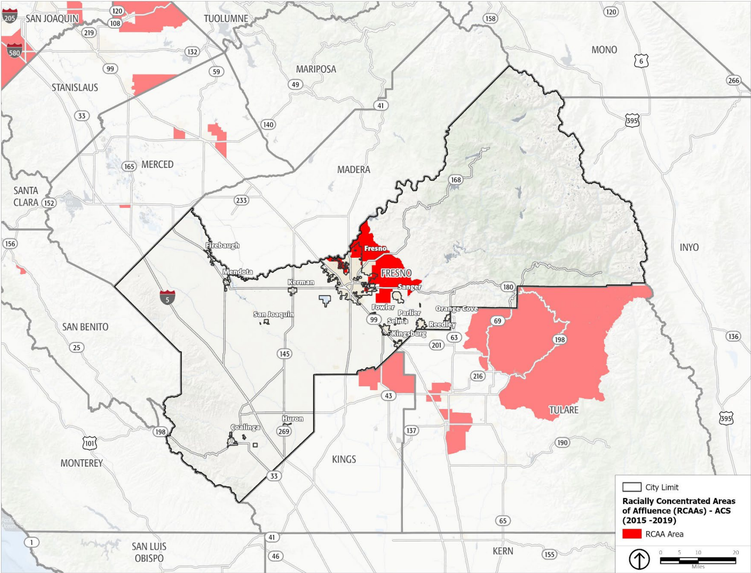
FIGURE 3-16 REGIONAL RCAAs
